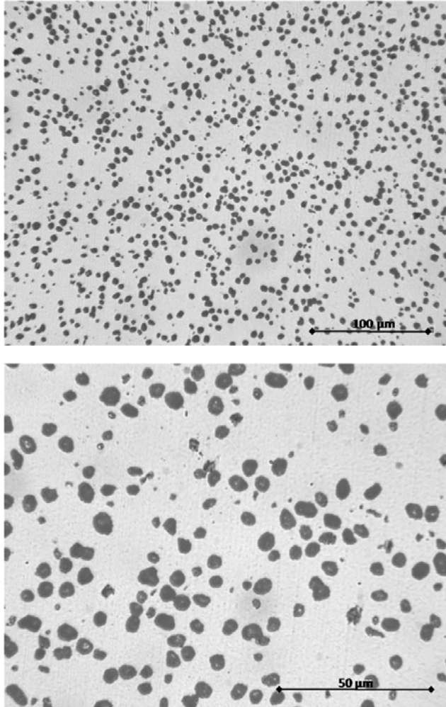
Figure 1. Alumina TCHP microstructure
