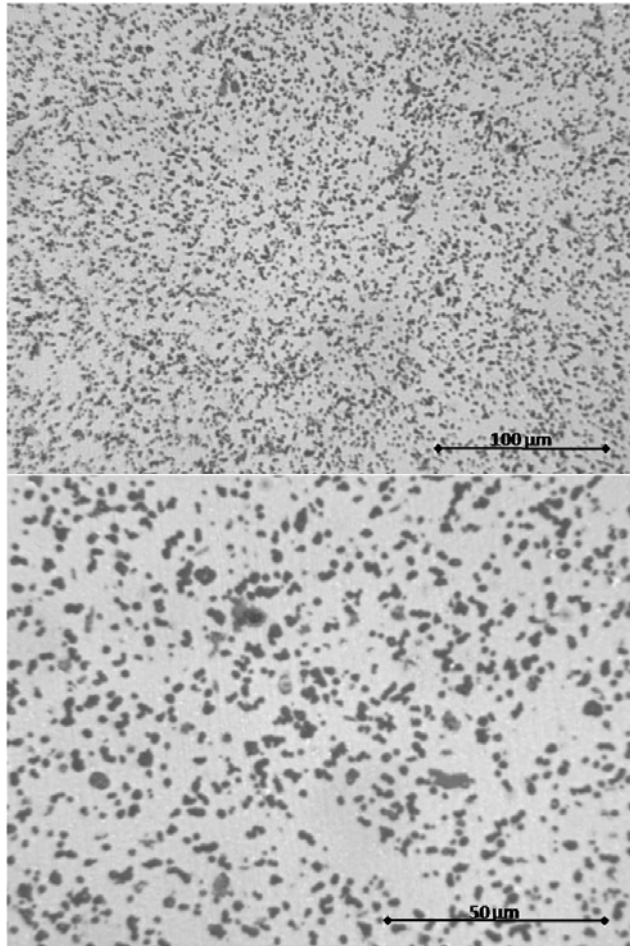
Figure 2. Titanium carbonitride TCHP microstructure
