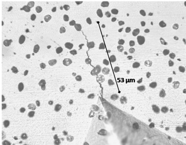
Figure 3. Resistance to crack propagation
